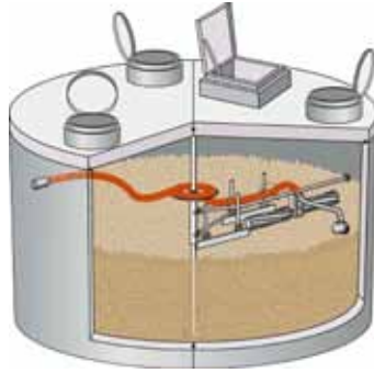
Plate 7: Large below-ground silo up to 60 m 3
