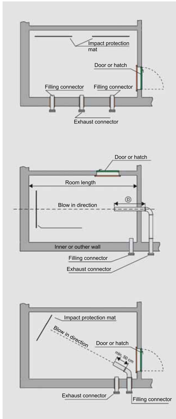
Plate 20 Special solutions for the filling system
